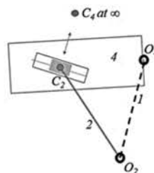
Equivalent Linkage
